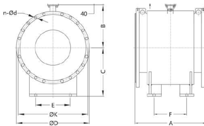
LMF11/12 Remote Type Sensor nominal size DN500 – DN2000
