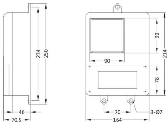
LMF11/12 Transducer (IP65) Sensor nominal size below DN500 refer LMF11
