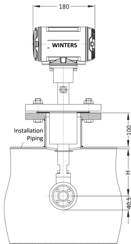
LMF14 Flange fixed type connection DN200 ~ 2000
